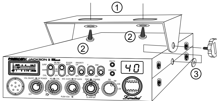
MOUNTING DIAGRAM
